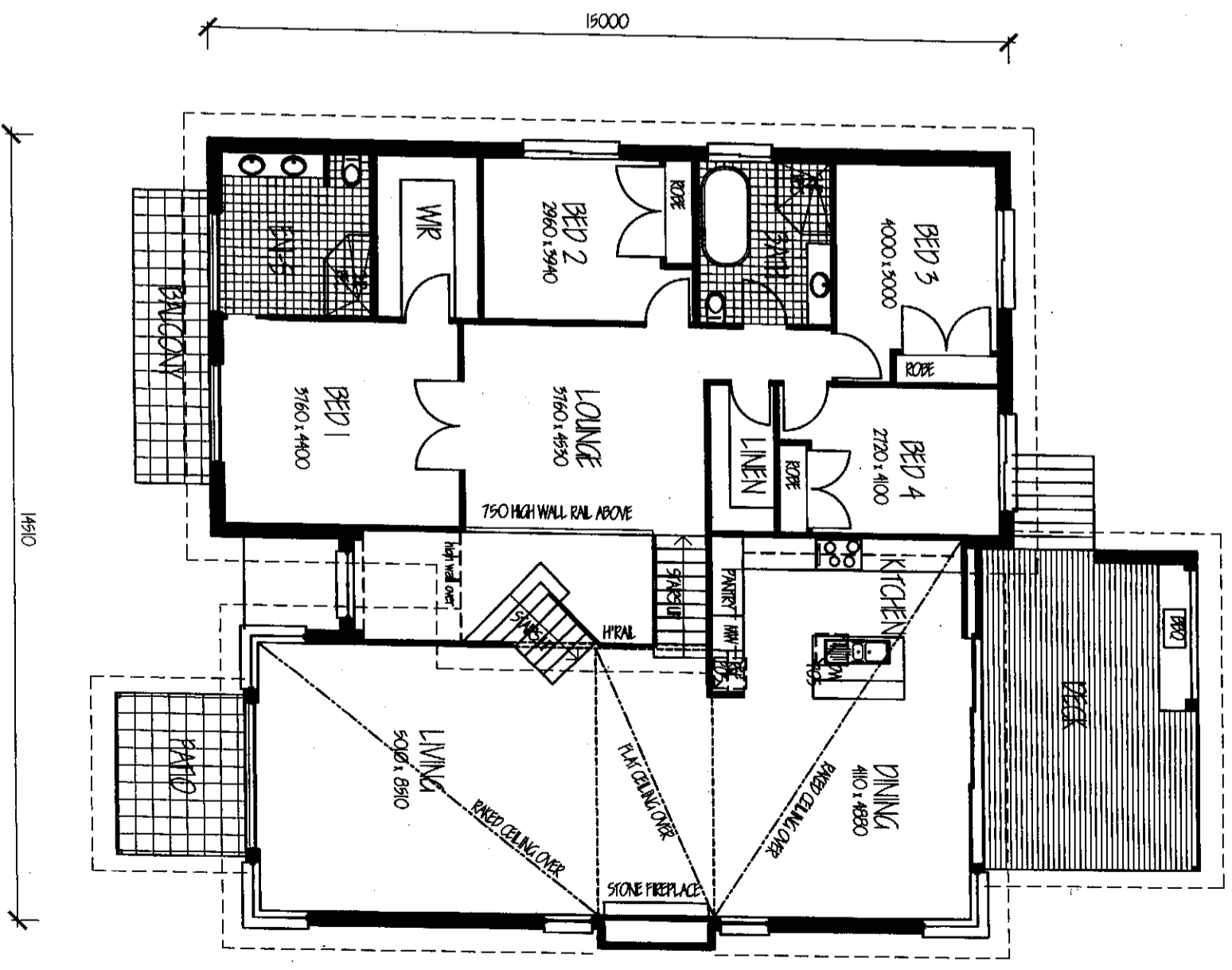
UPPER LEVELS PLAN
